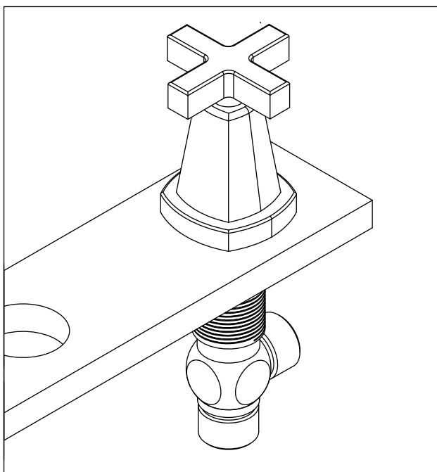
Install body from top of deck and twist to tighten
