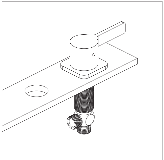
Tighten handle
