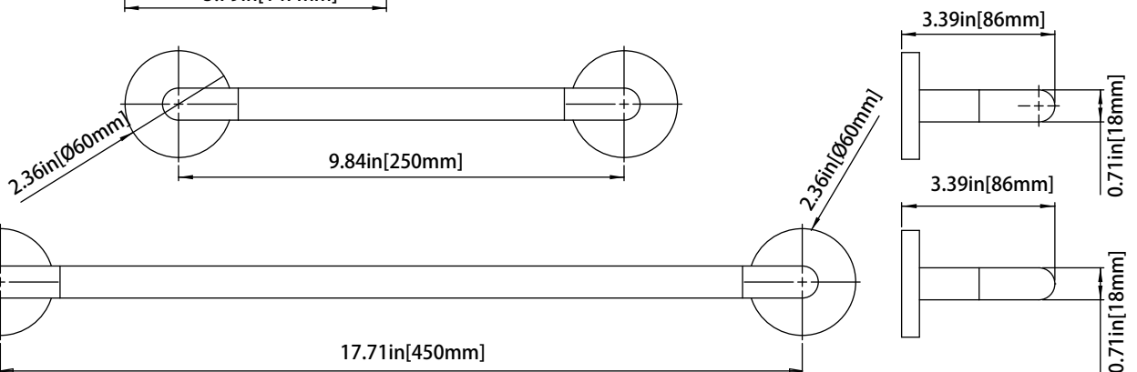
100.1009 Towel Bar - 18"
